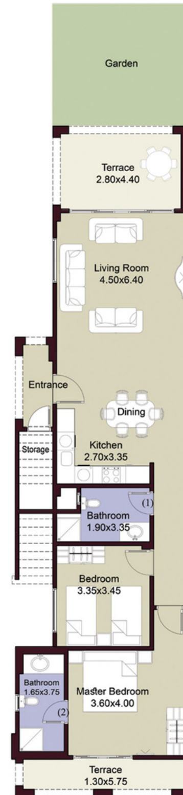
GROUND FLOOR
