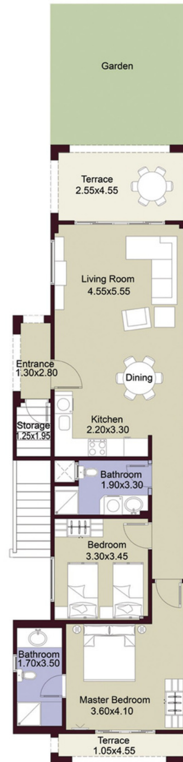
GROUND FLOOR
