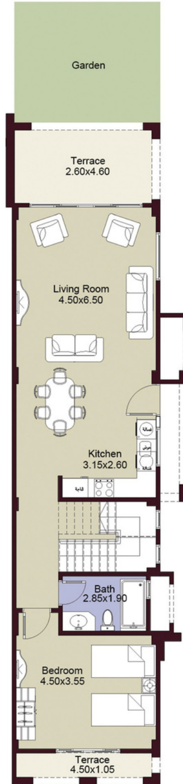
FIRST FLOOR
